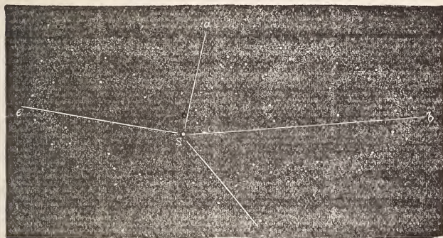
FIG. 8.—THE MILKY WAY REGARDED AS A SPIRAL.
